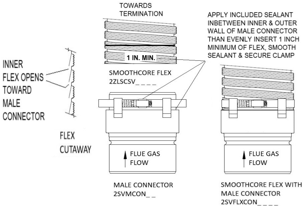
2SVMCON__ Male Connector & Sealant (field assembled)
