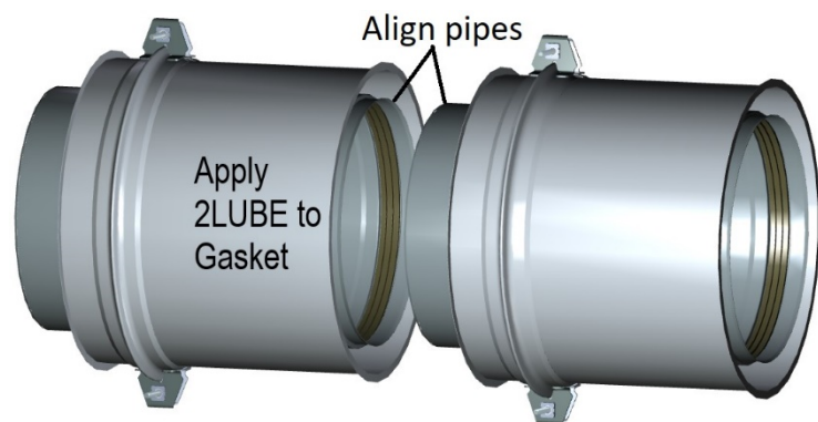
Double Wall ZV-Clamp Joint
