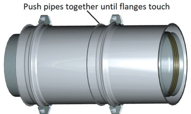
Double Wall ZV-Clamp Joint
