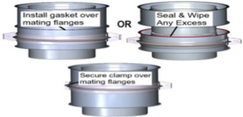
Z-Vent Double Wall with ZV-Clamp Installed Exterior to Building
